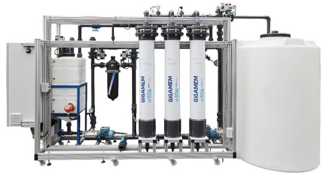
The C 2 -UF 30 HB system features three of Polymem's compact Gigamem® UF80G modules.
